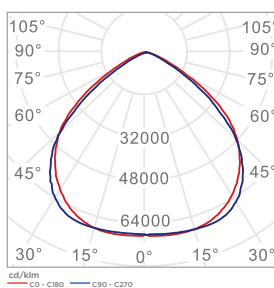
MDL-FLFB100W
