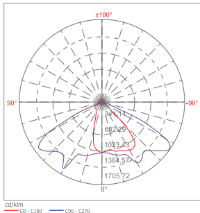
MDL-SL40W-03
