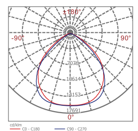
MDL-HB120W
